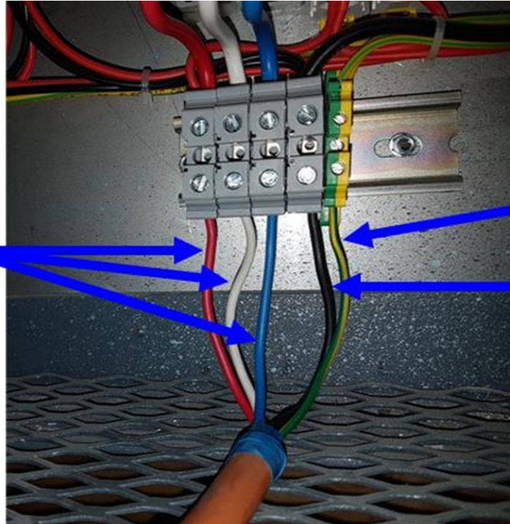
Wiring Cord Colour – Orange Flexible Cord (Older Kilns used Orange Flexible Cable and equipment wiring)
