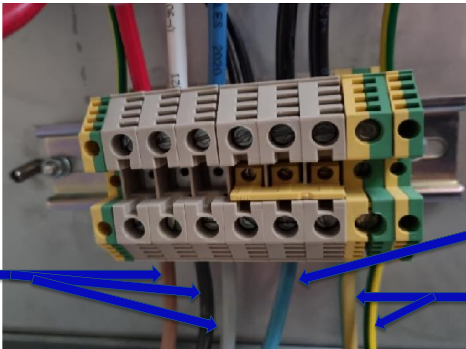
Wiring Cord Colour – Black Flexible Cord (European cables and current AS/NZS flexible cable and equipment wiring)
